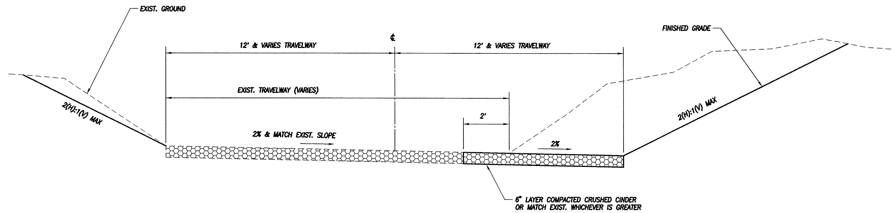
TYPICAL SECTION - EXCAVATION SHEET 7 - 8
