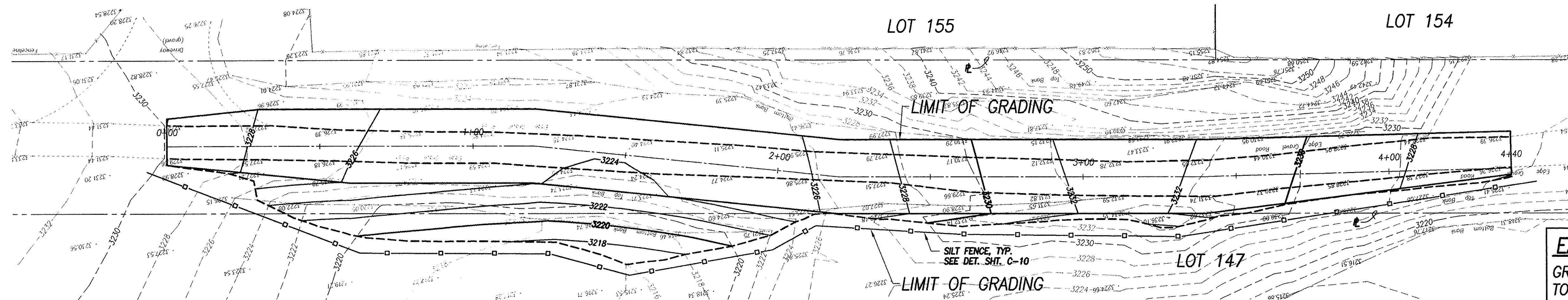
GRADING PLAN - FIRE ROAD 14 REPAIR SCALE: 1" = 20'
