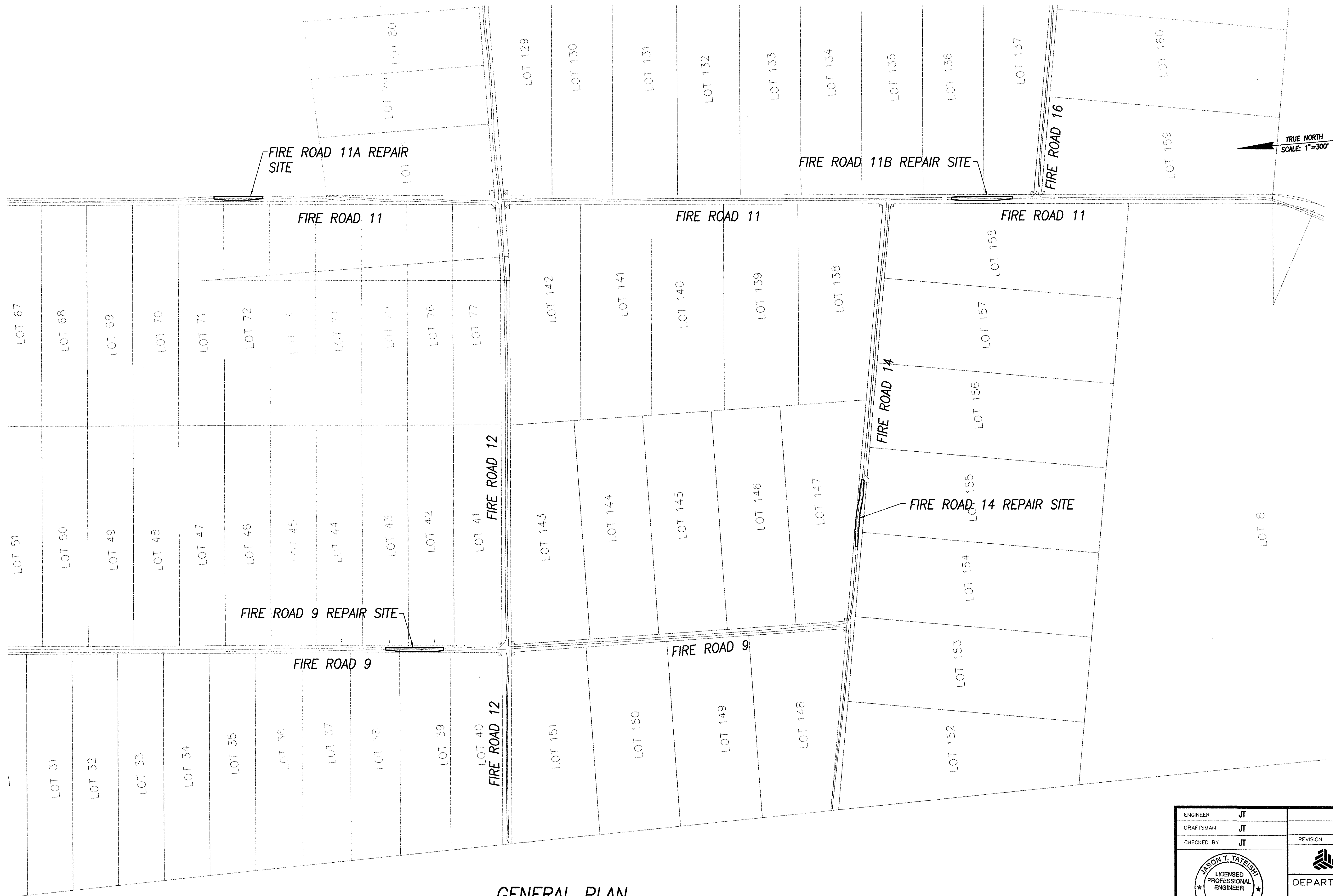
GENERAL PLAN SCALE: 1" = 300'
