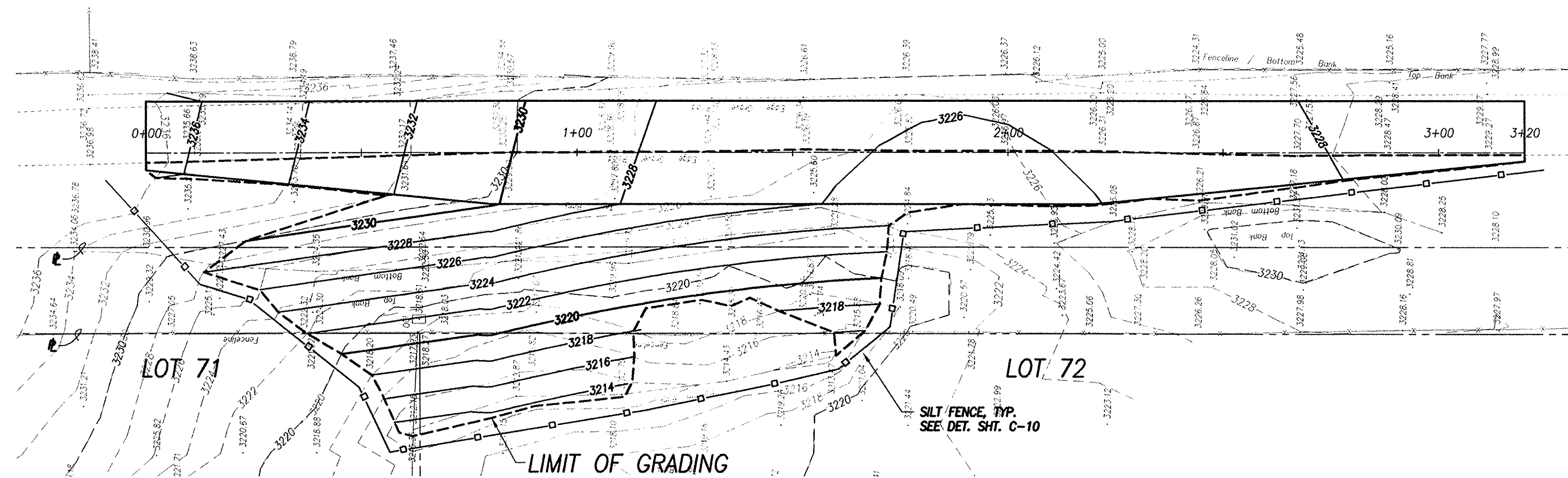
GRADING PLAN - FIRE ROAD 11A REPAIR SCALE: 1" = 20'
