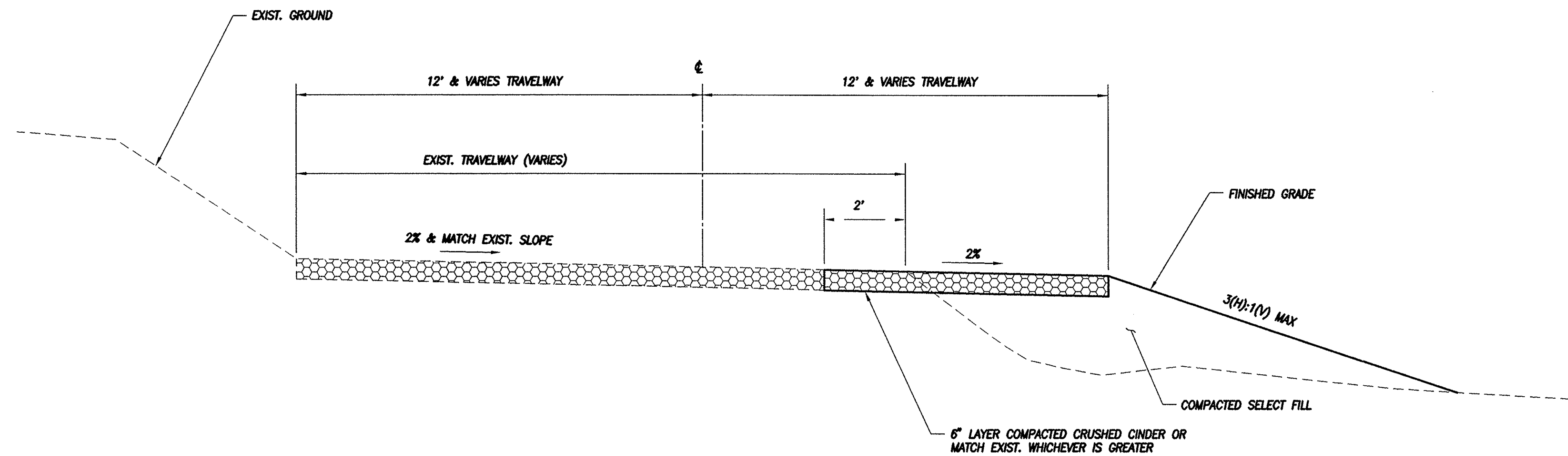
TYPICAL SECTION - EMBANKMENT SHEET 7 - 8
