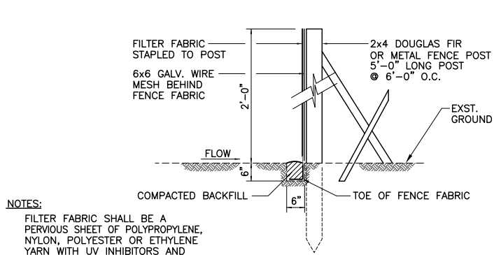
SECTION SILT FENCE NOT TO SCALE
