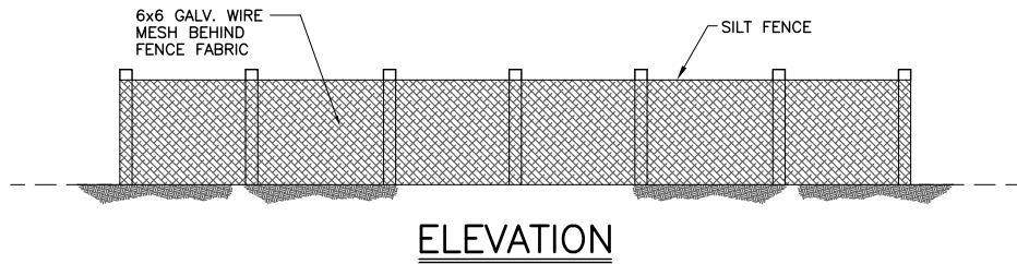
ELEVATION DETAIL SILT FENCE NOT TO SCALE
