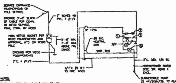
ONE-LINE DIAGRAM, WELL SITE NOT TO SCALE
