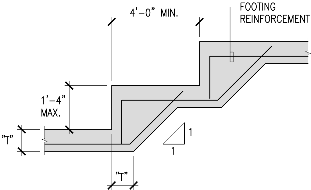
A TYP. STEPPED FOOTING S-101 NOT TO SCALE
