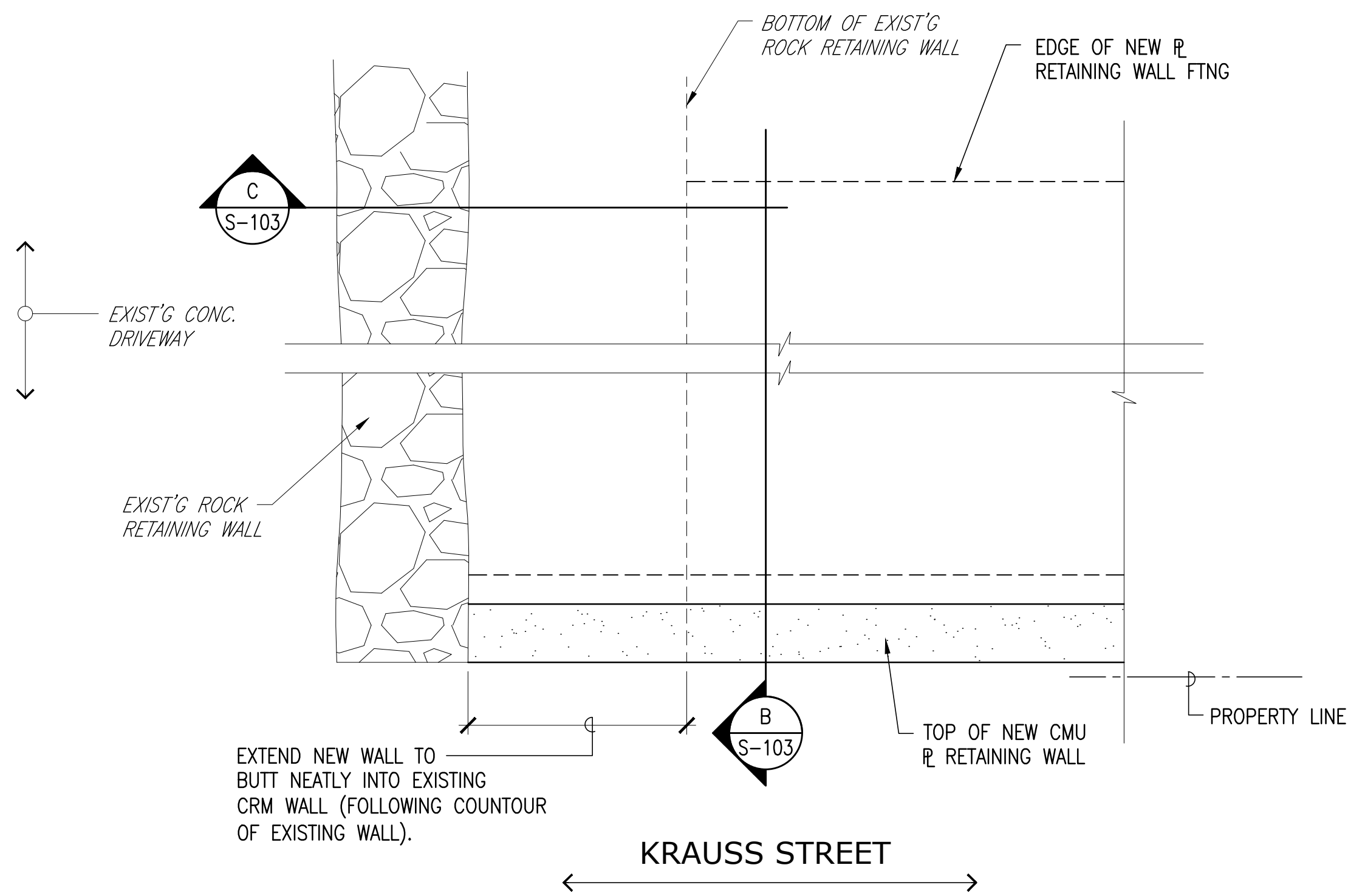
A PLAN VIEW DETAIL S-103 SCALE: NTS
