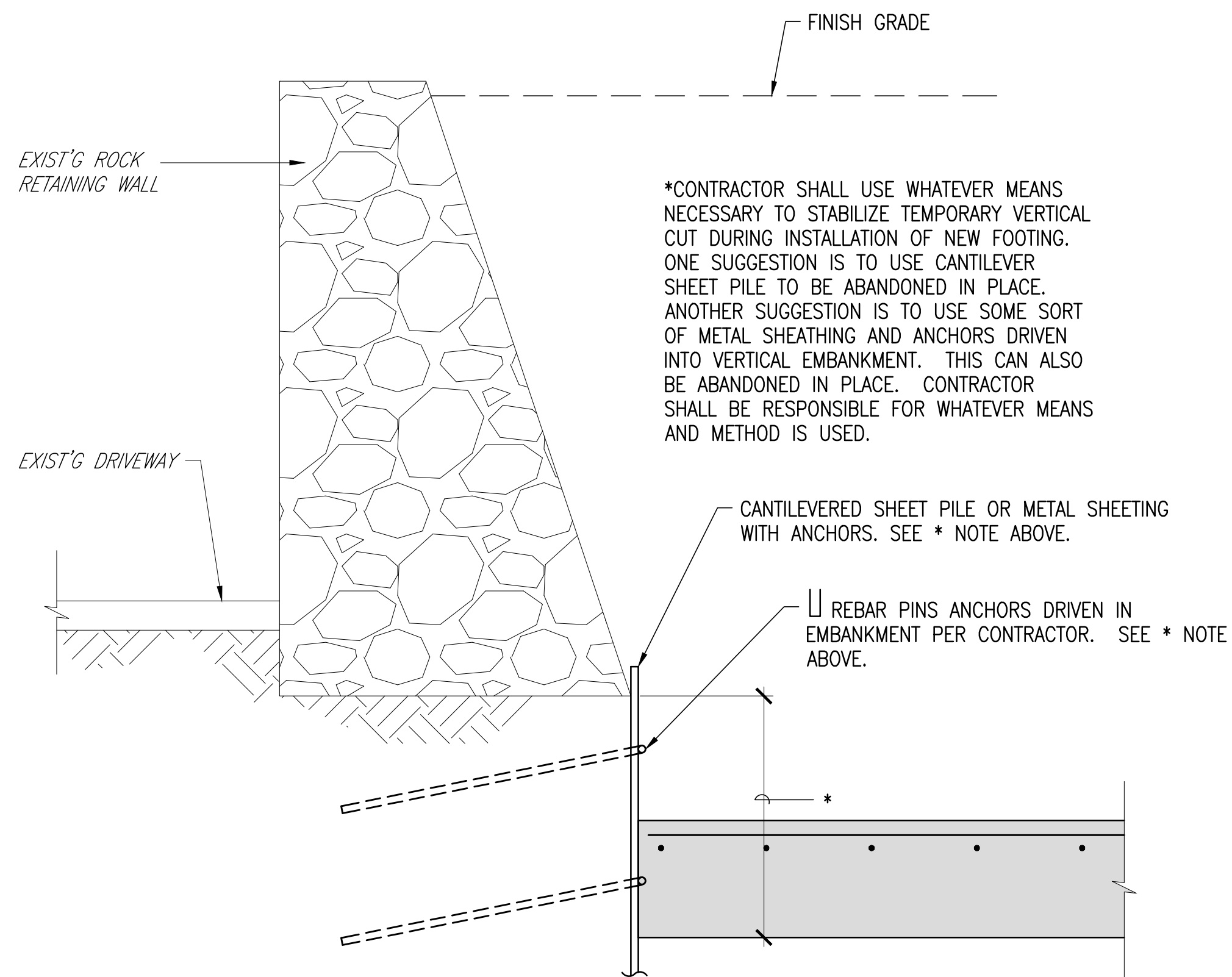
C SECTION - TEMPORARY CONDITION DURING NEW FOOTING CONSTRUCTION S-103 SCALE: NTS
