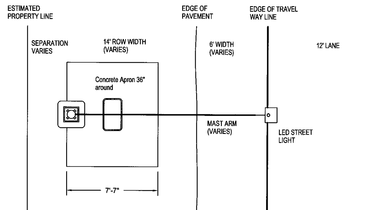
TYPICAL ARRANGEMENT FOR BARE GROUND WORK
